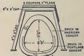
FIG. 7. IN 6" TUNNEL
